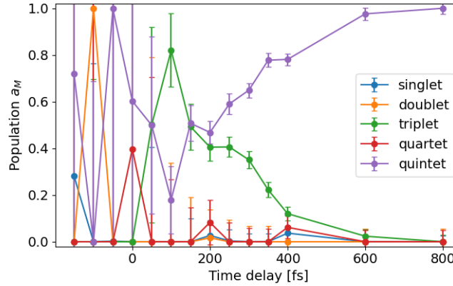
Figure 17: The population curves of the different spin states plotted against the time delay of the optical laser in femtoseconds.
