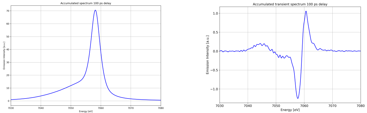
Figure 14: On the left the XES spectrum with the excitation laser on at a delay of 100 ps is plotted. On the right there's the difference spectrum at the same time delay.
