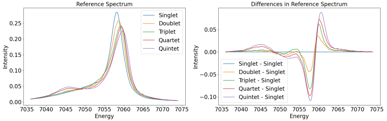
Figure 13: The reference spectra plotted with provided data for different spin states. The reference difference spectra with transient signals plotted with provided data for different transitions.
