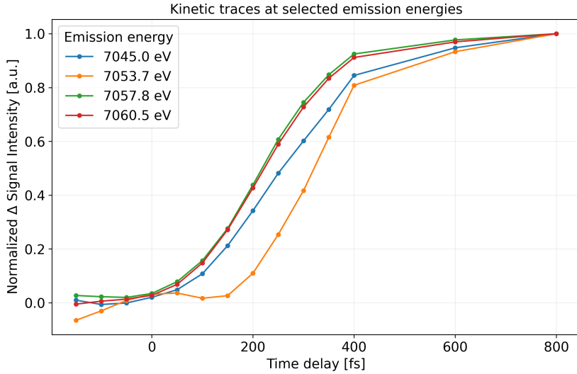
Figure 16: Kinetic traces at selected emission energies.
