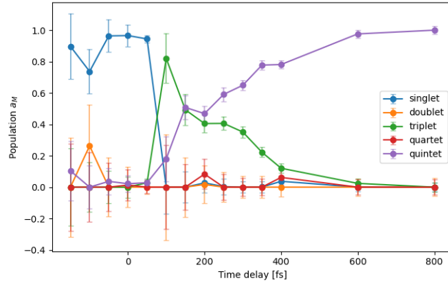
Figure 20: The adjusted population curves of the different spin states plotted against the time delay of the optical laser in femtoseconds.
