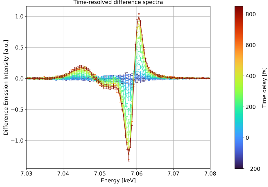
Figure 15: Transient spectra of the X-ray emission at different pump-probe time delays.
