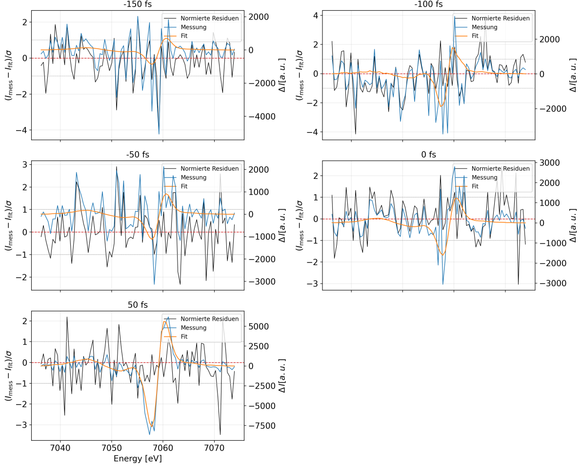
Figure 18: The normalised residuals together with the actual measurements and a fit over ... for time delays of \Delta t = \{-150 \text{ fs}, -100 \text{ fs}, -50 \text{ fs}, 0 \text{ fs}, 50 \text{ fs}\}
